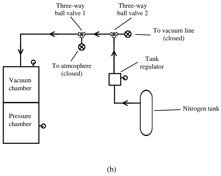
Figure 6.1 Diagram of the CFPS process, (a) during filling and (b) during pressurization. Arrows indicate the direction of airflow.
