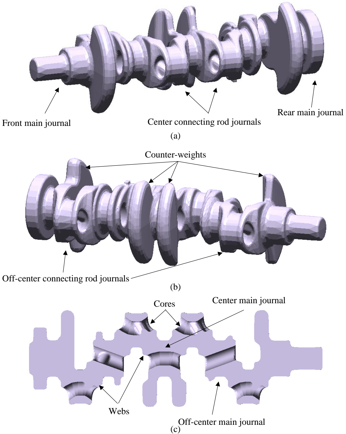
Figure 3.1 Geometry model of GM SGE cored crankshaft. (a) First isometric view, (b) second isometric view, (c) top view of a cut through the horizontal midplane. Various components of the crankshaft are labeled.
